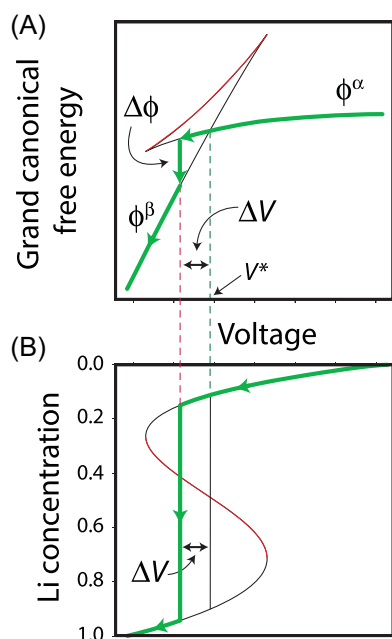
FIGURE 3 A first-order phase transformation can be analyzed in terms of the grand canonical free energy, \phi = g - x\mu_{Li} when controlling the voltage. (A) The grand canonical free energy for the free energy model of Figure 2B. The red portion corresponds to the unstable portion of the free energy in Figure 2B. The green line denotes a possible path when decreasing the voltage starting from the dilute \alpha phase. An overpotential \Delta V is always necessary to create a thermodynamic driving force \Delta\phi to overcome phase transformation barriers. (B) The need for a driving force \Delta\phi leads to a polarization of the plateau in the voltage curve that is equal to the overpotential \Delta V
